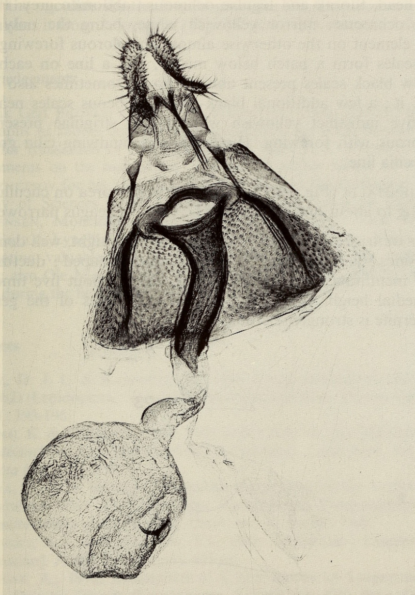
Fig. 22. Dichrorampha letarfensis GIBEAUX, female genitalia, prep. AJ1991.
