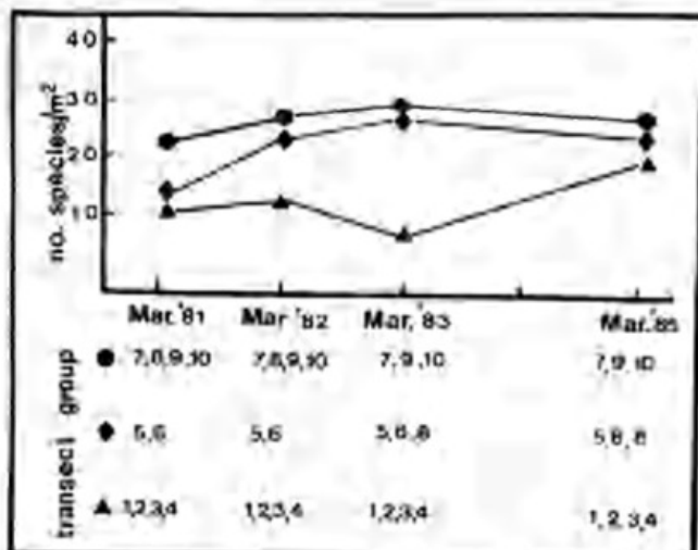
Fig. 6. Relationship between number of species/m 2 and transect group for the surveys of 1981-83 and 1985. All species were identified in these surveys.
