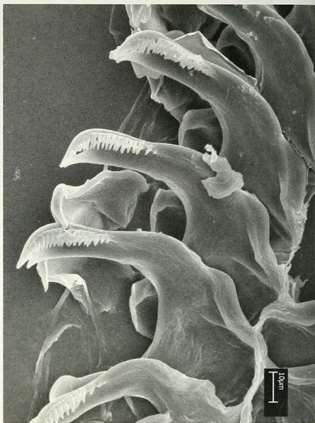
FIGURE 2. Okenia pellucida Burn, 1967 (CASIZ 078493). Scanning electron micrograph of radular teeth.
