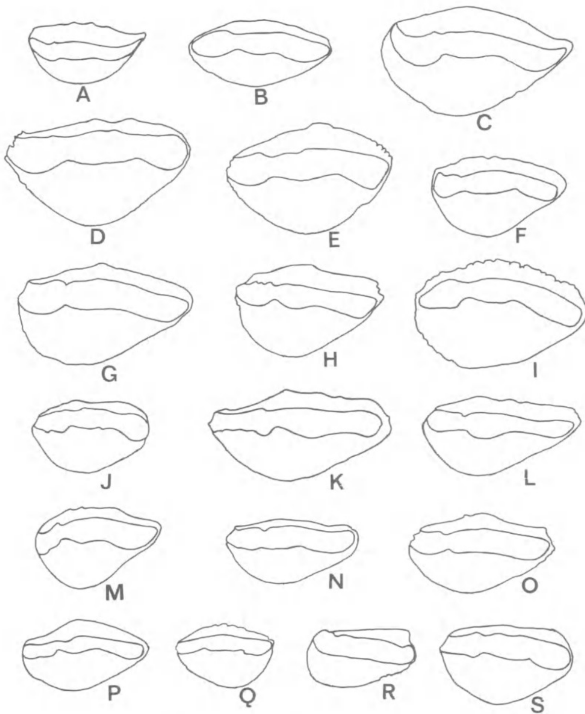
FIG. 14. Otoliths (right side) of A Sillago sihama , Madras, India. B . Sillago parvisquamis , Taiwan. C . Sillago vincenti , India. D,E . Sillago ciliata , Sydney. F . Sillago analis , Shark Bay. G . Sillago maculata maculata , New South Wales. H . Sillago maculata burrus , Shark Bay. I . Sillago maculata aeolus , Singapore. J . Sillago bassensis bassensis , Western Australia. K . Sillago bassensis flindersi , New South Wales. L . Sillago vittata , Shark Bay. M . Sillago robusta , New South Wales. N . Sillago robusta , Western Australia. O . Sillago schomburgkii , Shark Bay. P . Sillago ingenua , Thailand. Q . Sillago japonica , Tokyo. R . Sillaginopsis panijus , Bay of Bengal. S . Sillaginodes punctata , South Australia.
