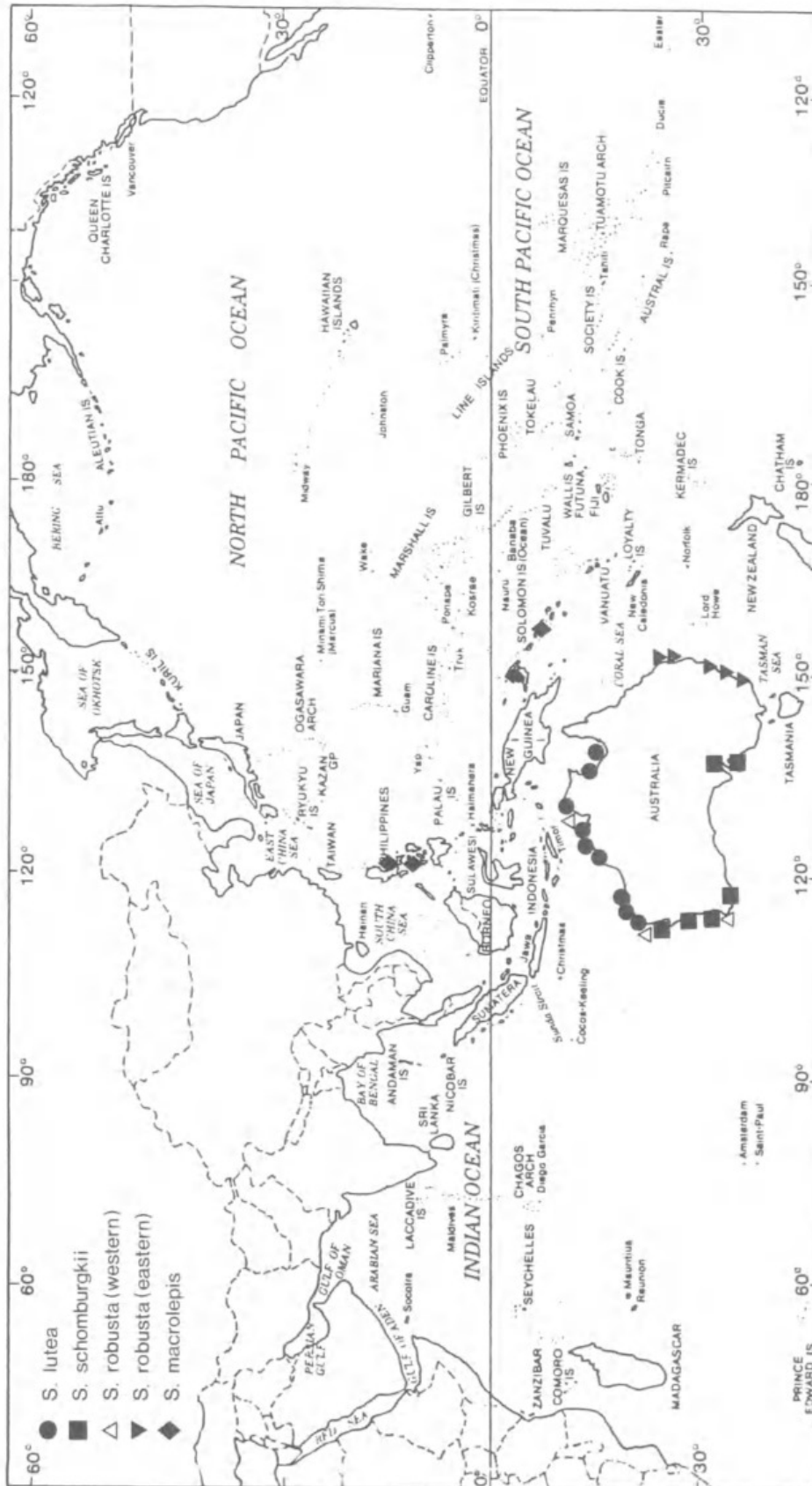
FIG. 18. Distributional records for Sillago , species.
