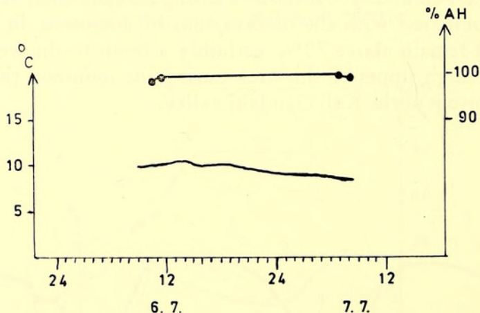
Diagram 14: Temperature (lower line) and airhumidity (upper line) deeply underneath rocks in a burrow system of Alticola stoliczkanus located in the Syang Kola valley, 4210 m.
