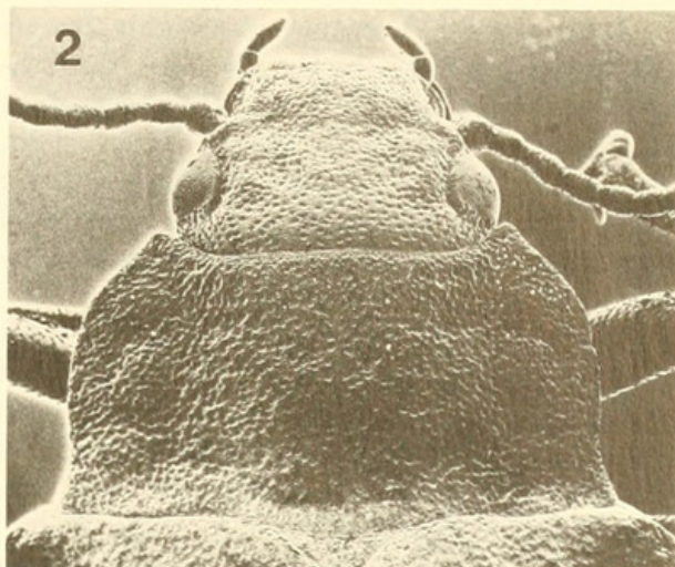
FIGURE 2. Amphizoa davidi Lucas: scanning electron micrograph of head and pronotum, dorsal aspect, magnification = 25 \times (specimen uncoated).
