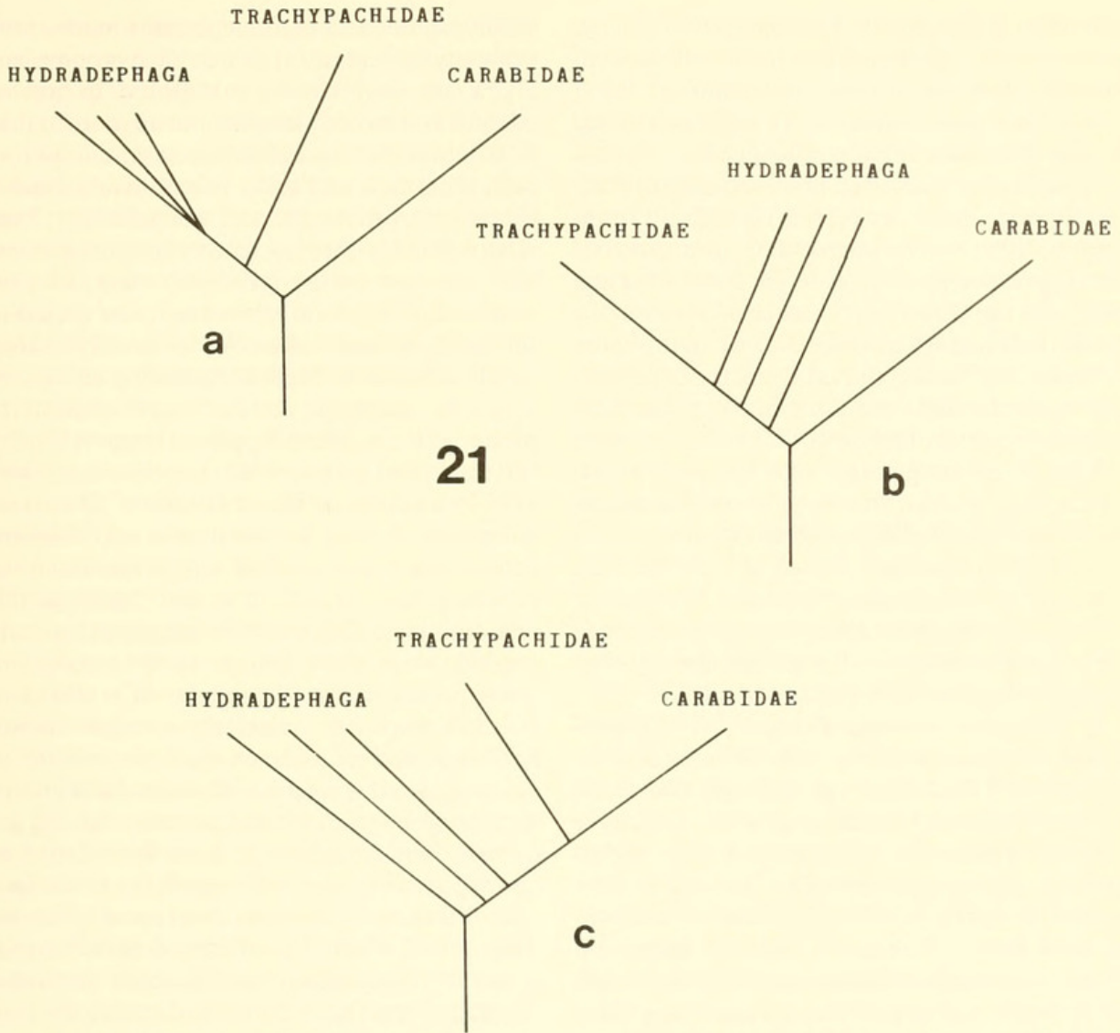
FIGURE 21. Illustrations of alternative hypotheses of phylogenetic relationships among Hydradeephaga, trachypachids, and carabids.
