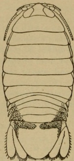
FIG. 6.— ROCINELA BELLICEPS (STIMPSON). \times 2\frac{1}{2} .
