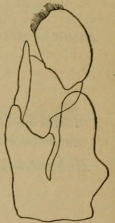
FIG. 24. — MAXIL- LIPED OF CLEANTIS OCCIDENTALIS. GREATLY ENLARGED
