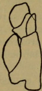
FIG. 22.—MAXILLIPED OF COLIDOTEA ROSTRATA (BENEDICT).
