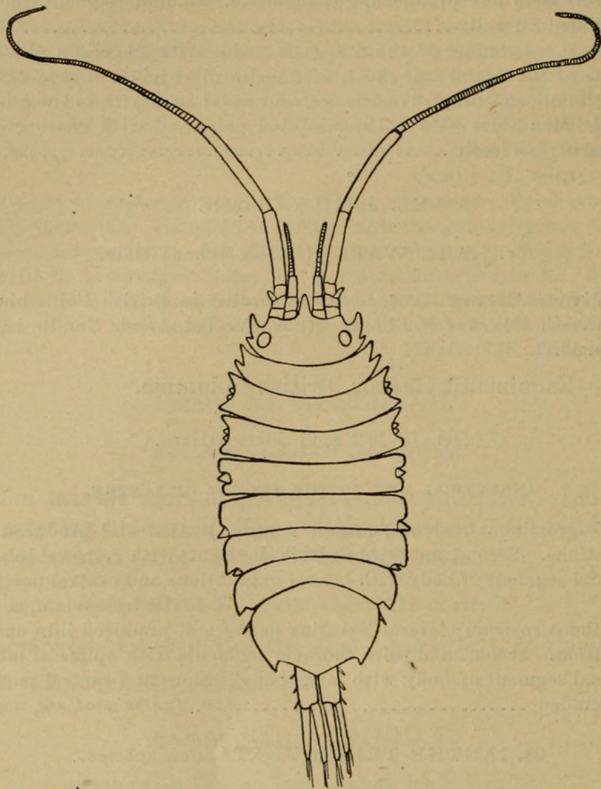
FIG. 29.— IANTHE TRIANGULATA . \times 13\frac{1}{2} .
