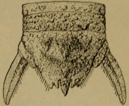
FIG. 18.— CILICÆA GRANULOSA . × 8. LAST THORACIC SEGMENT AND ABDOMEN.
