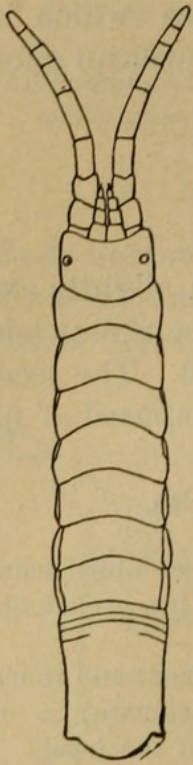
FIG. 25.—CLEANTIS HEATHII. \times 6\frac{2}{3} .
