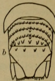
FIG. 4.—CORALLANA TRUNCATA. \times 13\frac{1}{2} . a , HEAD; b , ABDOMEN AND LAST THORACIC SEGMENT.
