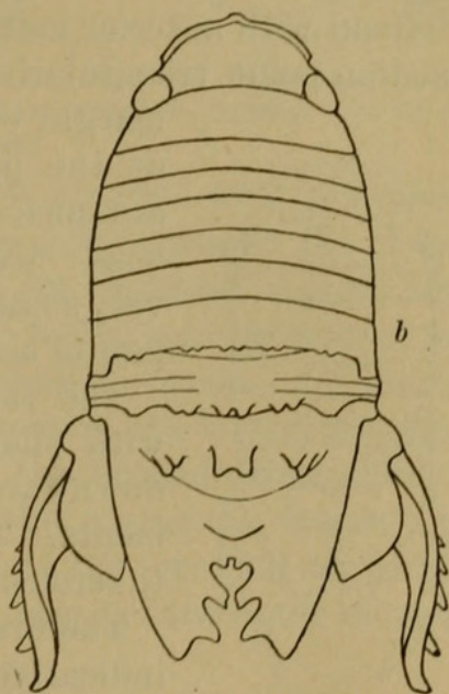
FIG. 16.— CILICÆA CORDATA . \times 8 . a, HEAD AND FIRST THORACIC SEGMENT; b, DORSAL VIEW.
