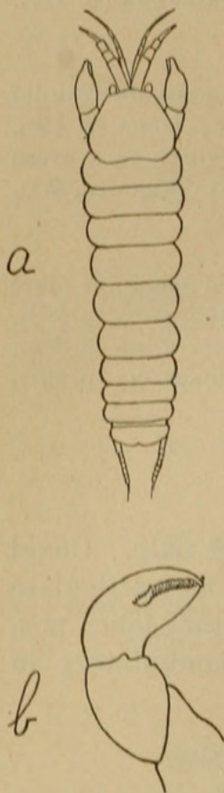
FIG. 1.— TANAIS ALASCENSIS , NEW SPECIES. × 8. a , DORSAL VIEW; b , LAST TWO JOINTS OF LEG OF THE FIRST PAIR.
