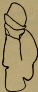
FIG. 27.—MAXILLIPED OF EUSYMMERUS ANTENNATUS.
