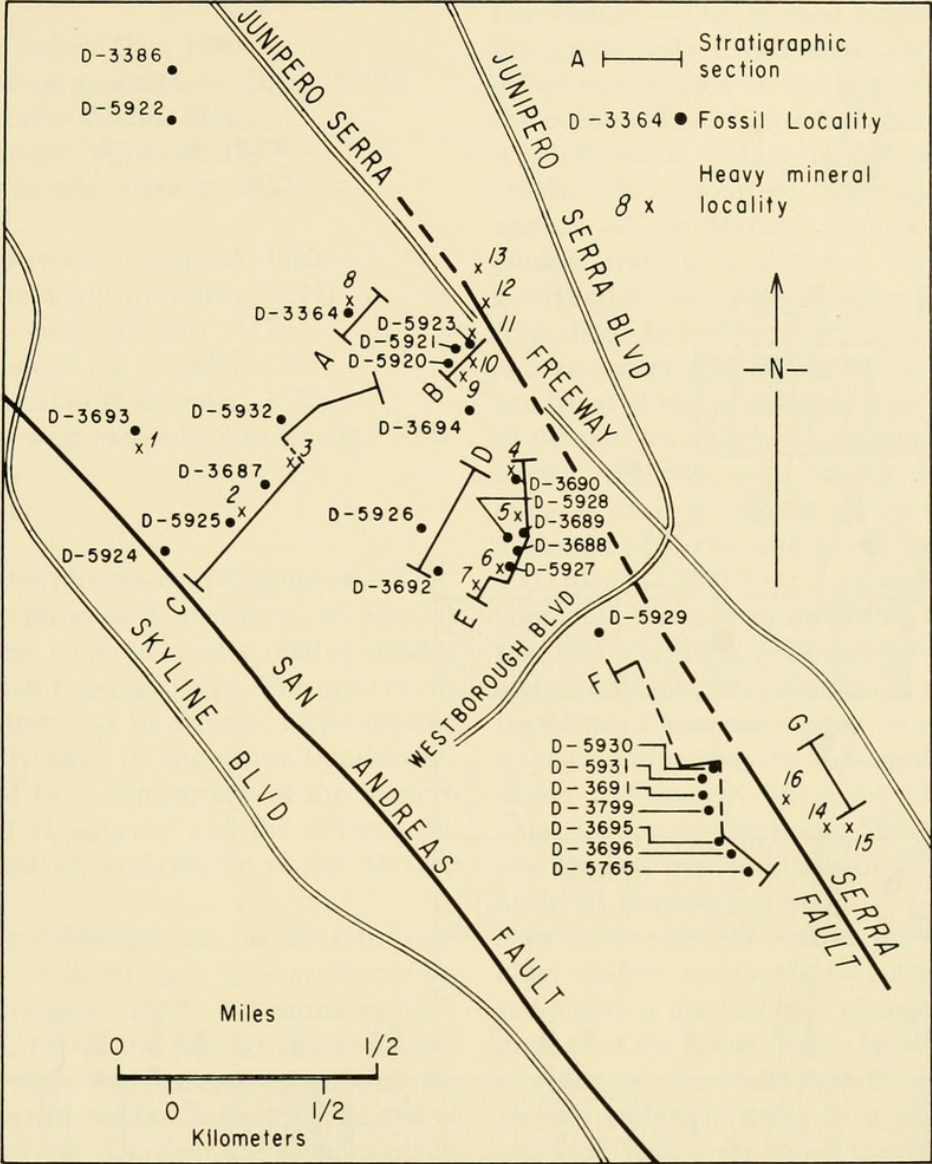
FIGURE 2. Location map of stratigraphic sections, fossil locations, and heavy mineral sample locations in the Twelvemile Creek area.
