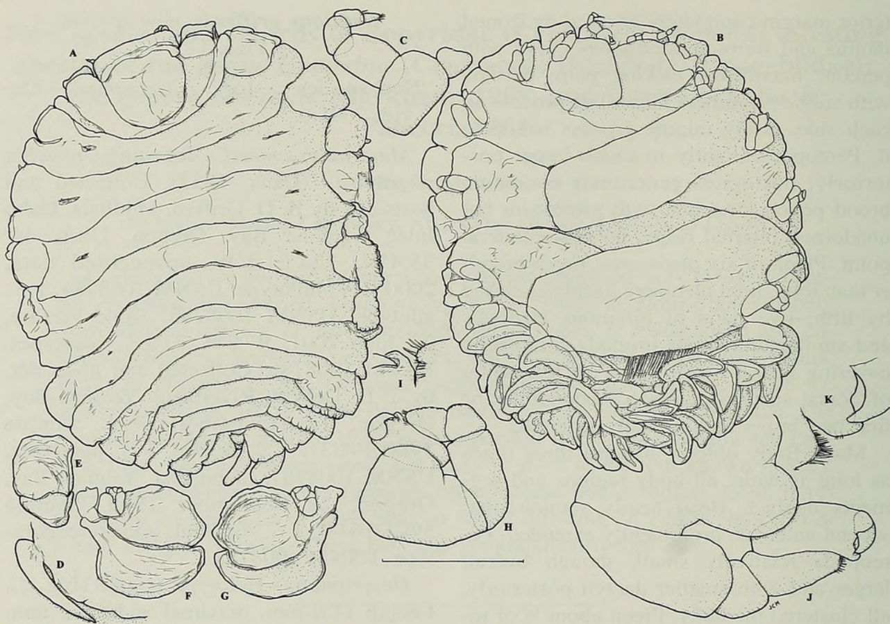
Fig. 1. Orthione griffenis , new species. Holotype female. A. Dorsal. B. Ventral. C. Right antennae. D. Right side of barbula. E. Right maxilliped. F. Right oostegite 1, external. G. Same, internal. H. Right pereopod 1. I. End carpus and dactylus of same. J. Right pereopod 7. K. End carpus and dactylus of same. Scale: 3.60 mm for A, B, E–G; 1.20 mm for C; 2.40 mm for D; 1.00 mm for H, J; 0.4 mm for I, K.
