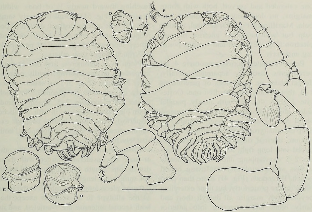
Fig. 4. Orthione mesoamericana , new species. Holotype female. A. Dorsal. B. Ventral. C. Right antennae. D. Right maxilliped. E. Pleuron of same. F. Right side of barbula. G. Right oostegite 1, external. H. Same, internal. I. Right pereopod 1. J. Right pereopod 7. Scale: 2.00 mm for A, B, D, F–H; 1.00 mm for E; 0.36 mm for C, I, J.
