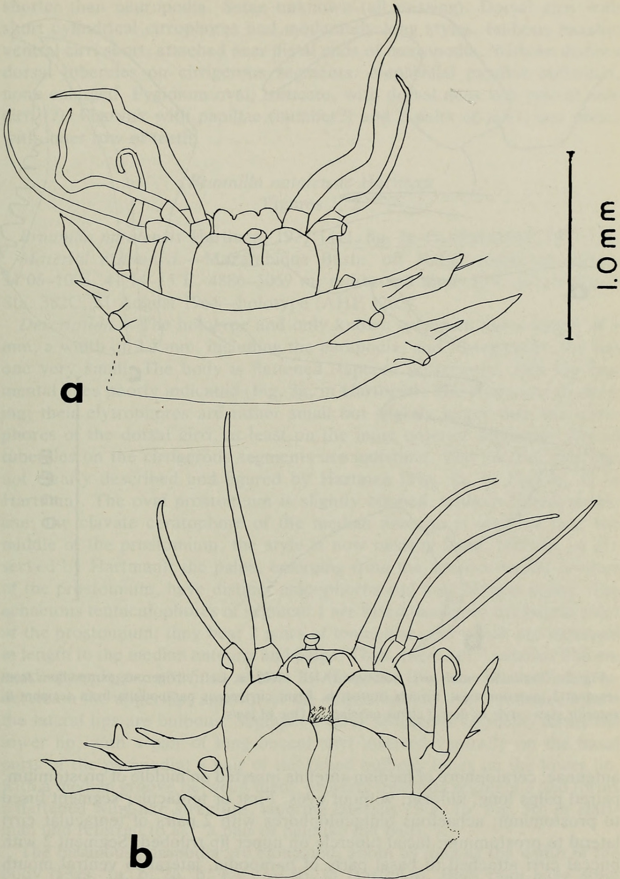
Fig. 1. Bruunilla natalensis , holotype (AHF 1202): a , Dorsal view of anterior end; left parapodium of segment 3 had been cut off; styles of median antenna, right dorsal tentacular cirrus, right buccal cirrus of segment 2, right dorsal cirrus of segment 3 and elytra of segment 2 missing; b , Ventral view of same; left margin of wing-like structure overlapping segment 3 damaged.
