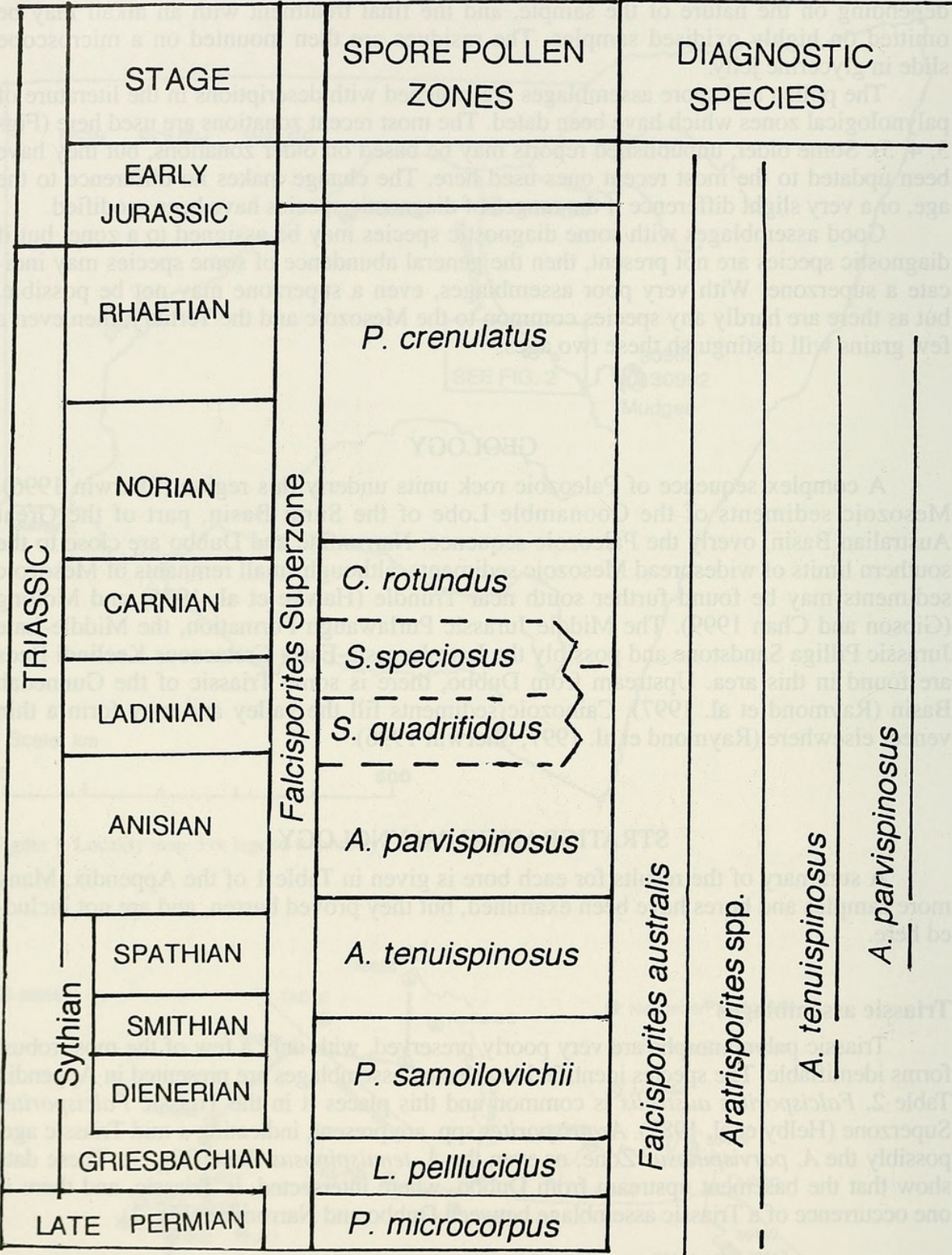
Figure 3. Range chart for Triassic species. From Helby et al. (1987).
