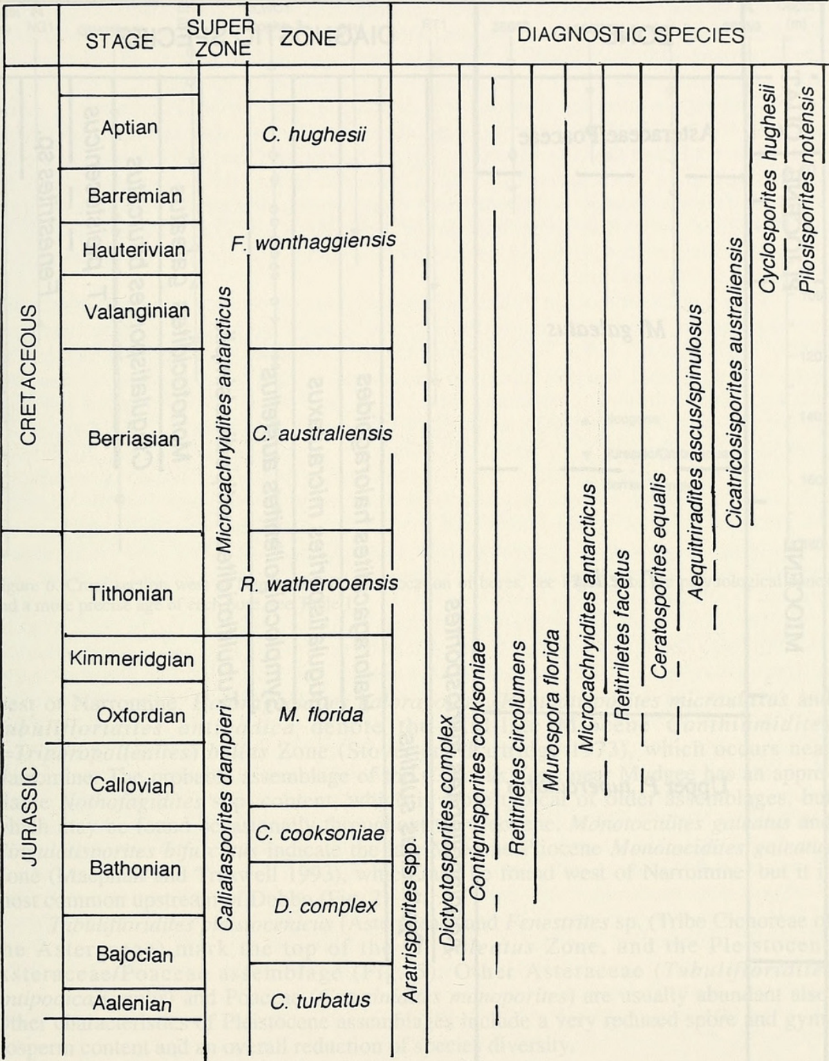
Figure 4. Range chart for the Mid-Late Jurassic and Early Cretaceous. From Helby et al. (1987).
