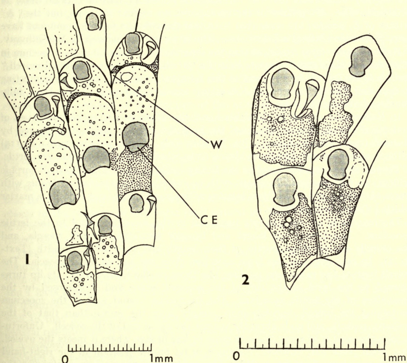
FIGS. 1 AND 2. Neoeuthyris woosteri (MacGillivray), 1948.3.12.1.
