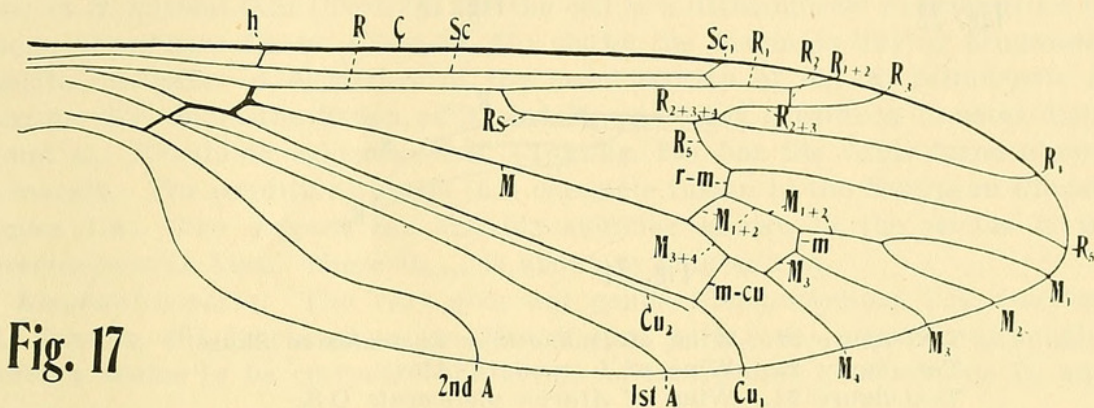
Text-figure 17. Wing of Gynoplistia bella Walk.
