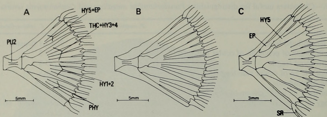
Fig. 5. Caudal skeletons: A, Cephalopsetta ventrocellata , ANSP 153379, 161.7 mm SL; B, Pseudorhombus megalops , HUMZ 111769, 146.5 mm SL; C, Ancylosetta quadrocellata , FDNR 6115, 52.9 mm SL; abbreviations: EP = epural; HY 1–5 = hypurals 1–5; PHY = parhypural; PU2 = preural centrum 2; SR = splinter ray; THC = terminal half-centrum.
