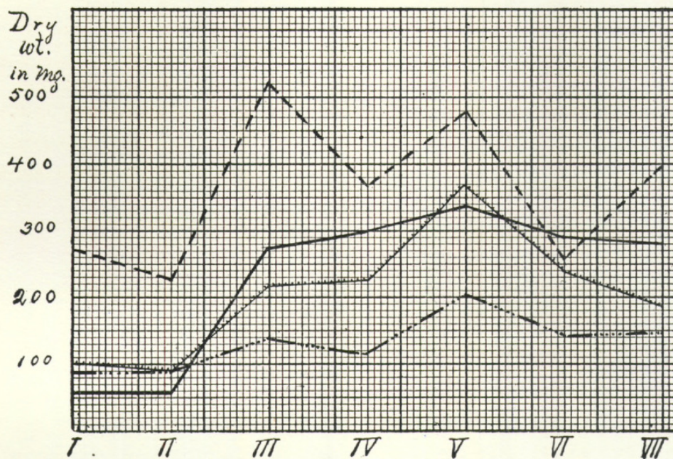
Fig. 3. Glomerella Gossypii ; dry weights of cultures in mg. on ordines, solutions (see p. 166 for explanation) on abscissae. Key to graphs in fig. 1.
