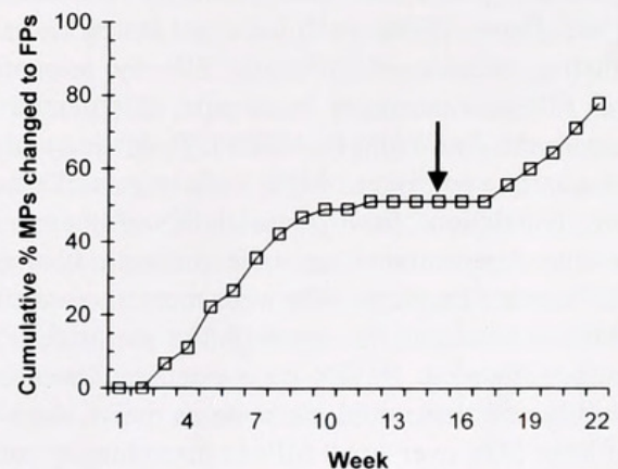
Figure 5. Change of large MPs to FPs in the suboptimal treatment during 22 weeks, first under suboptimal temperature and photoperiod for 14 weeks (as in Fig. 4A) and then after a change to optimal conditions (arrow) for the next 8 weeks.
