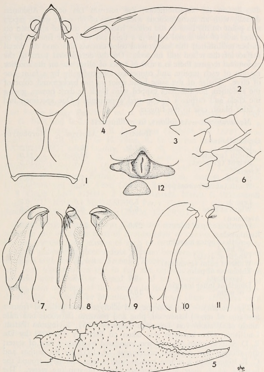
Figures 1 - 12. Procambarus planirostris , sp. nov.: 1, 2, cephalothorax of the holotype; 3, epistome of the holotype; 4, antennal scale of the holotype; 5, chela and carpus of the holotype; 6, hooks on ischiopodites of the third and fourth pereopods of the holotype; 7, 8, 9, mesial, caudal and lateral views of the first pleopod of the holotype; 10, 11, mesial and lateral views of the morphotype; 12, annulus ventralis of the allotype. Pubescence removed from all structures illustrated.
