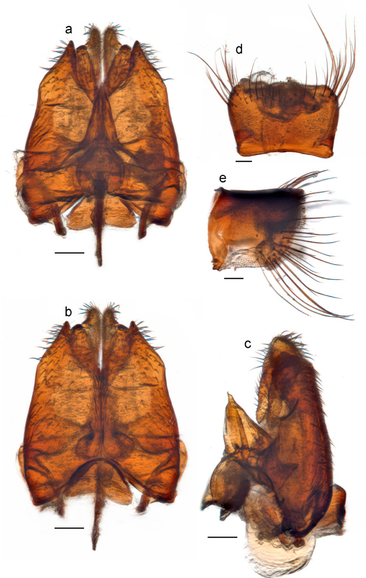
Figure 22. Thevenetimyia nigrapicalis (Roberts, 1929) ♂ genitalia: (a) genital capsule, dorsal; (b) genital capsule, ventral; (c) genital capsule, lateral; (d) epandrium, dorsal; (e) epandrium, lateral. Scale bars = 0.1 mm.
