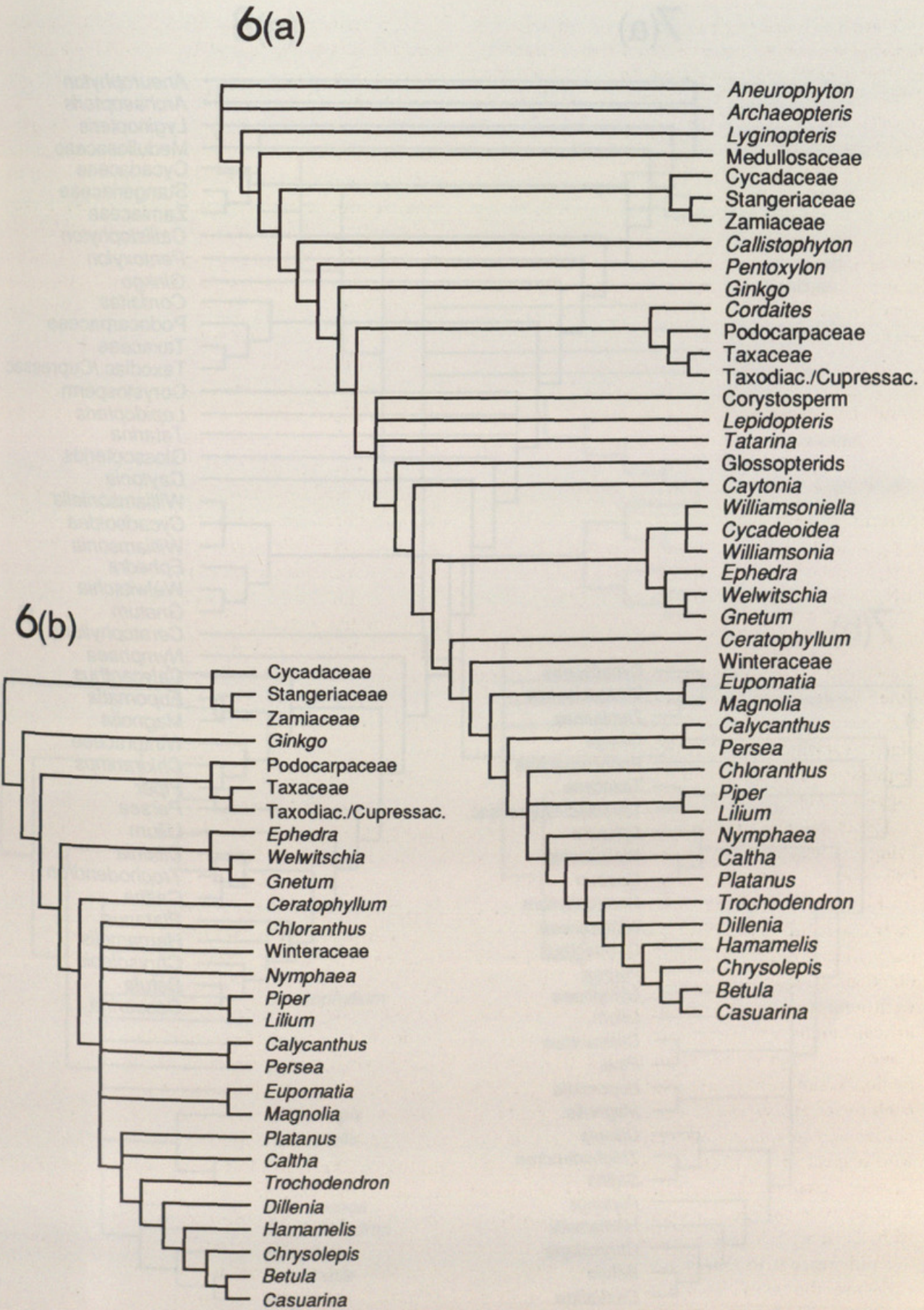
FIGURES 6-8. Total evidence analyses of morphological and rbcL data for fossil and extant seed plants. The morphological data and taxon sampling of Nixon et al. (1994; matrix version as of 8 November 1993) was followed for cladistic analyses of fossil and living seed plants (the "a" series) and of extant seed plants only (the "b" series). For both taxonomic scopes, rbcL evidence was combined as one of three data forms: nucleotide sequences (6), nucleotide string recognitions (7), or amino acid sequences (8) obtained from single organisms (see Table 2). For
