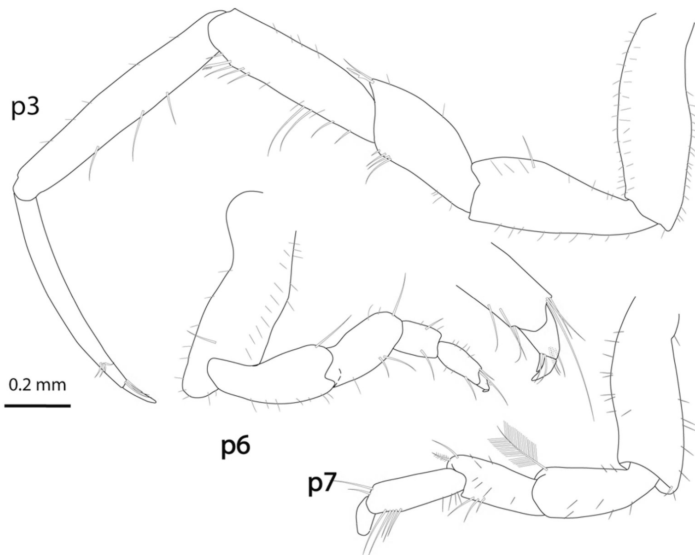
Figure 4. Zenobianopsis cidaris sp. nov. Right limbs from holotype; detail of p6 untwisted.
