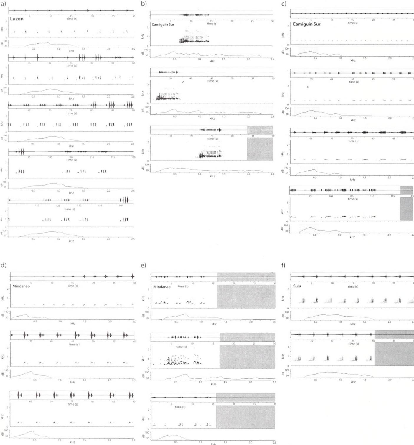
Figure 2. Typical songs of each major taxon in the Philippine Hawk Owl Ninox philippensis ( sensu lato ) complex. For each song, the first row is the waveform, the second is the sonagram, and the third is the spectrum: (a): Philippine Hawk Owl N. p. philippensis , probably non-duetted long song of single bird singing in different directions, hence the variations in amplitude late in the song series; AV#2171, PCR, Luzon; (b): Camiguin Hawk Owl Ninox new species 1, duetted series of short strophes; AV#13554, ROH, Camiguin Sur; (c): Camiguin Hawk Owl Ninox new species 1, long song by single bird; AV#13622 ROH, Camiguin Sur; (d): Mindanao Hawk Owl N. spilocephala , long song by single bird (series continued in SOM 1j); NSA Wildlife ref. #132605, S. Harrap, Mindanao; (e): Mindanao Hawk Owl N. spilocephala , short duetted songs; AV#12461, ROH, Mindanao; (f): Sulu Hawk Owl N. reyi , series of short probably non-duetted strophes; AV#14577, ROH, Tawi Tawi; (g): Mindoro Hawk Owl, first half of long duet (continued in SOM 1l); AV#11507, ROH, Mindoro; (h): long song of single Romblon Hawk Owl Ninox spilonota new subspecies; AV#10803, DNSA, Tablas; (i–j): long song of single Romblon Hawk Owl N. spilonota on Sibuyan, AV#13637, ROH, Sibuyan; (k): long song of single Cebu Hawk Owl Ninox new species 2, AV#12612, BD, Cebu; (l): duetted song of Cebu Hawk Owl Ninox new species 2; AV#10805, LMP, Cebu.
