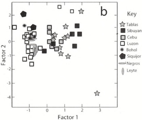
Figure 3. Results of PCAs of measurements of vocal characteristics for (a) all groups ( philippensis and centralis combined) and (b) core groups ( philippensis and centralis from different islands graphed separately; Tablas spilonota , Sibuyan spilonota , and Cebu).
