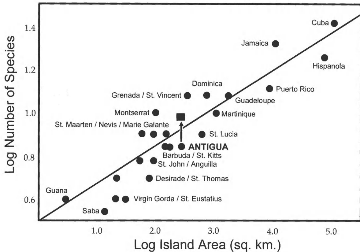
Figure 2. Species/area curve for the chiropteran fauna in the Antilles. Data are from Genoways et al. (2001) with minor modification. Linear regression of log-transformed data: y = 0.17x + .49 ( R^2 = 0.81 ). For argument (see text), Antigua has been represented twice with the extant complement of seven species of bats (closed circle) and with its complement increased by three additional species (Arrow: Square).
