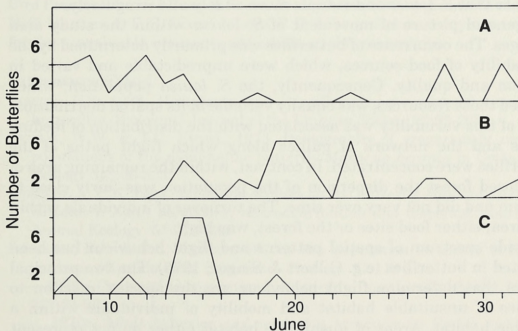
Fig. 4 The number of Stichophthalma lousia observed flying along gullies. No records were made on 16 and 22 June due to bad weather. A section 77, gully with a brook; B section 74, dry gully; C section 70, dry gully.
