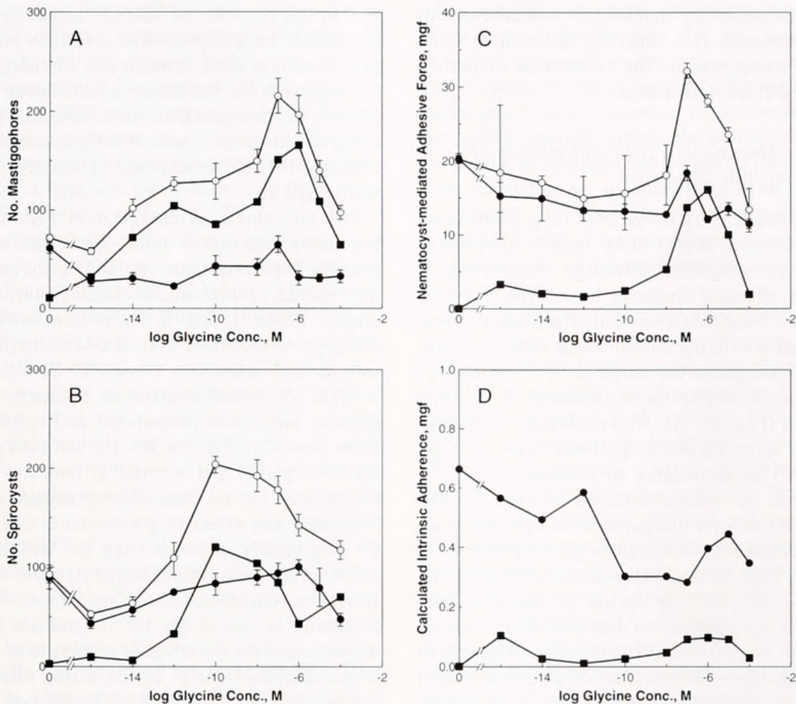
Figure 3. Afferent and efferent cnida dose-responses to glycine. Combined responses from Type B plus Type C cnidocyte/supporting cell complexes (CSCCs) are measured in seawater (open circles). Cnida responses from Type Cs only are measured in the presence of 10^{-8} M D-600 in seawater (closed circles). Calculated responses from Type Bs (closed squares) are obtained by subtracting Type C responses from combined Type B plus Type C responses. Values express the mean of duplicate experiments. Each experiment consists of replicate probes for each glycine concentration; each probe and each tentacle is used only once. Vertical bars represent standard error of the mean and are applied to all measured means, but not to calculated means. (A) Effect of glycine on nematocyst discharge ( n = 15 ). (B) Effect of glycine on spirocyst discharge ( n = 15 ). (C) Effect of glycine on nematocyst-mediated adhesive force ( n = 14 ). (D) Effect of glycine on calculated intrinsic adherence.
