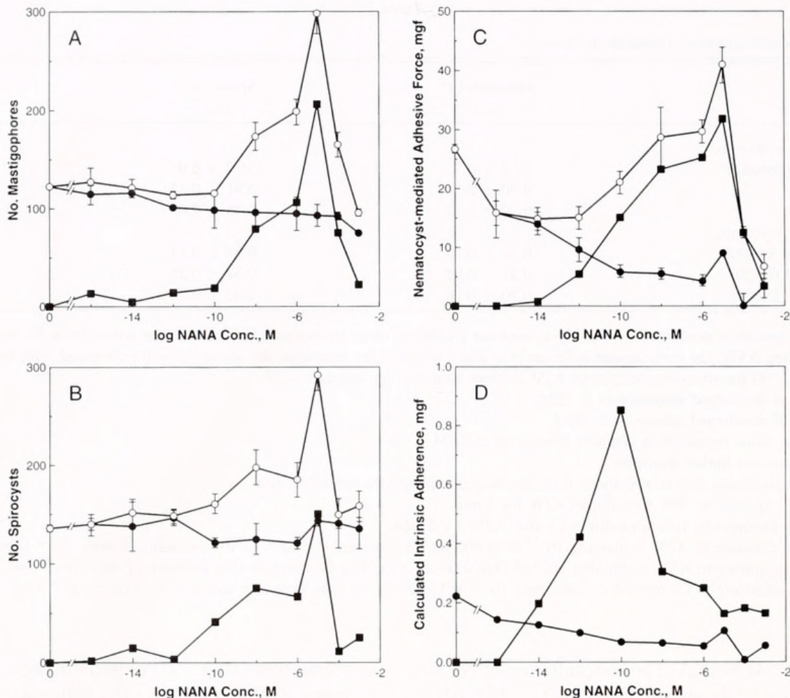
Figure 2. Afferent and efferent cnida dose-responses to N-acetylneuraminic acid (NANA). Combined cnida responses from Type B plus Type C cnidocyte/supporting cell complexes (CSCCs) are measured in seawater (open circles). Cnida responses from Type Cs only are measured in the presence of 10^{-10} M D-600 (closed circles). Calculated responses from Type Bs (closed squares) are obtained by subtracting Type C responses from combined Type B plus Type C responses. Values express the mean of three experiments. Each experiment consists of replicate probes for each NANA concentration; each probe and each tentacle is used only once. Vertical bars represent standard errors of the mean and are applied to all measured means, but not to calculated means. (A) Effect of NANA on nematocyst discharge ( n = 34 ). (B) Effect of NANA on spirocyst discharge ( n = 35 ). (C) Effect of NANA on nematocyst-mediated adhesive force ( n = 36 ). (D) Effect of NANA on calculated intrinsic adherence.
