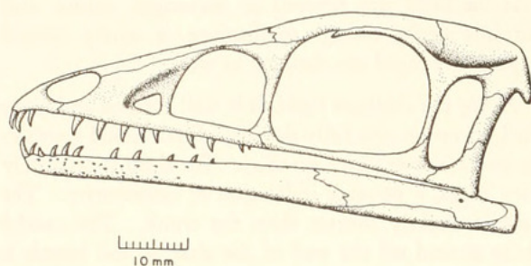
Figure 3: Reconstruction of the skull and jaws of Compsognathus longipes . The temporal region is largely hypothetical, as are the sutural details between the maxilla, jugal and lacrymal, the jugal and post-orbital, and the quadrate-jugal, quadrate and squamosal. The number of teeth shown is the absolute minimum, recording only those that are preserved in place or are indicated by tooth impressions. Empty alveoli due to tooth replacement or post mortem loss cannot be distinguished. The diastema at the premaxilla — maxilla suture is real.
