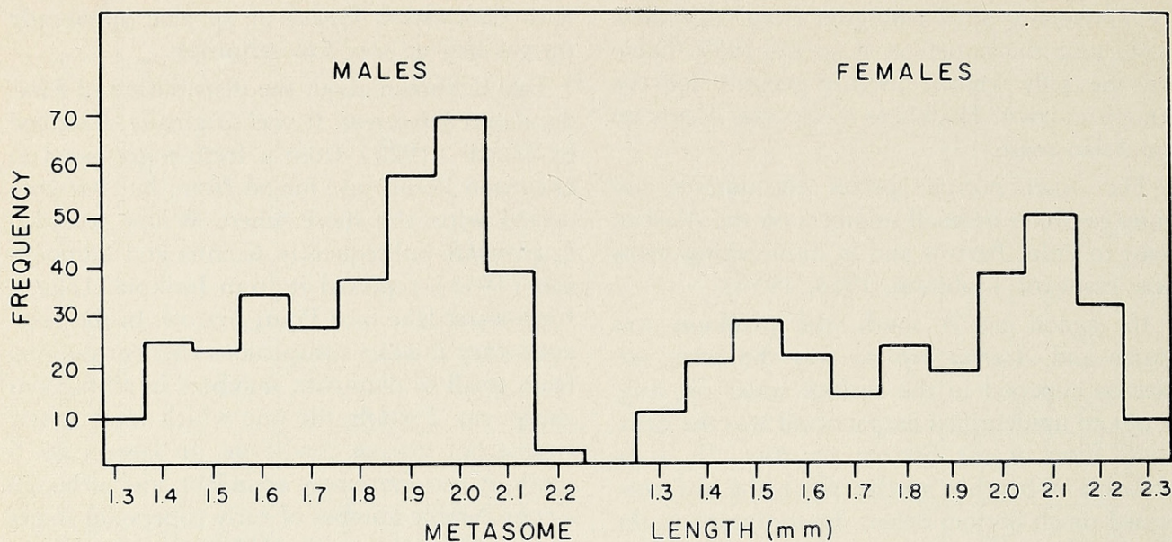
FIG. 2. Length frequency histogram for Limnocalanus johanseni adult (copepodid VI) population.
