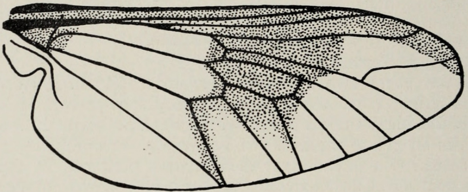
Fig. 1. Chrysops patricia Pechuman n. sp. Wing.
