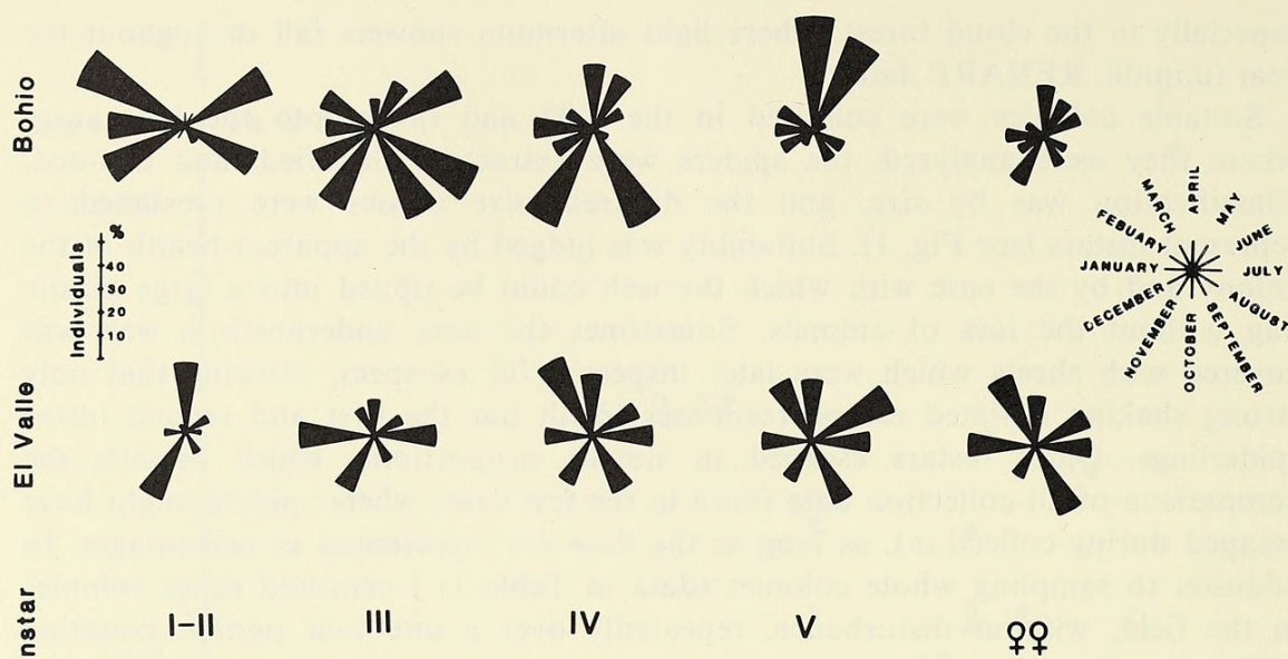
Fig. 3.—Size class composition of colonies collected in the lowland (Bohio) and the highland sites (El Valle). Each circular histogram represents the annual cycle (reading clockwise), the length of each sector gives the relative proportion of spiders (in percent) of the particular size class (indicated by the roman numeral) at the sampling month (compare Table 1).
