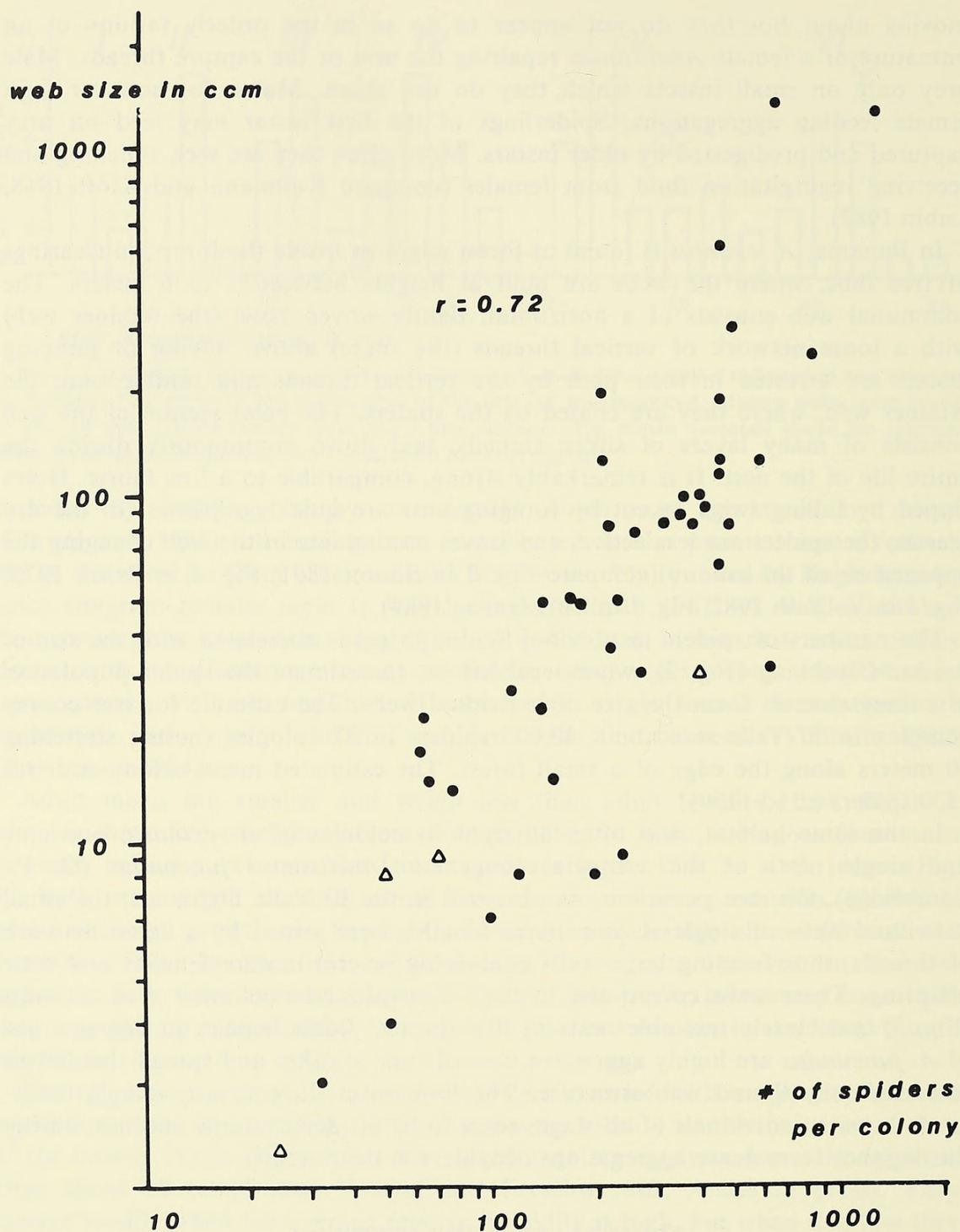
Fig. 2.—Scattergram and correlation coefficient ( r ) of the size (volume) of the retainer web and the number of Anelosimus eximius inhabiting it. Volume was calculated using the equation 2/3 \pi a^2 b ( a = height of bowl, b = width, c = length of bowl). The formula of the regression line was y = x^a + b . Each point represents one colony of A. eximius , the triangles represent colonies of the subsocial congeneric A. juncundus .
