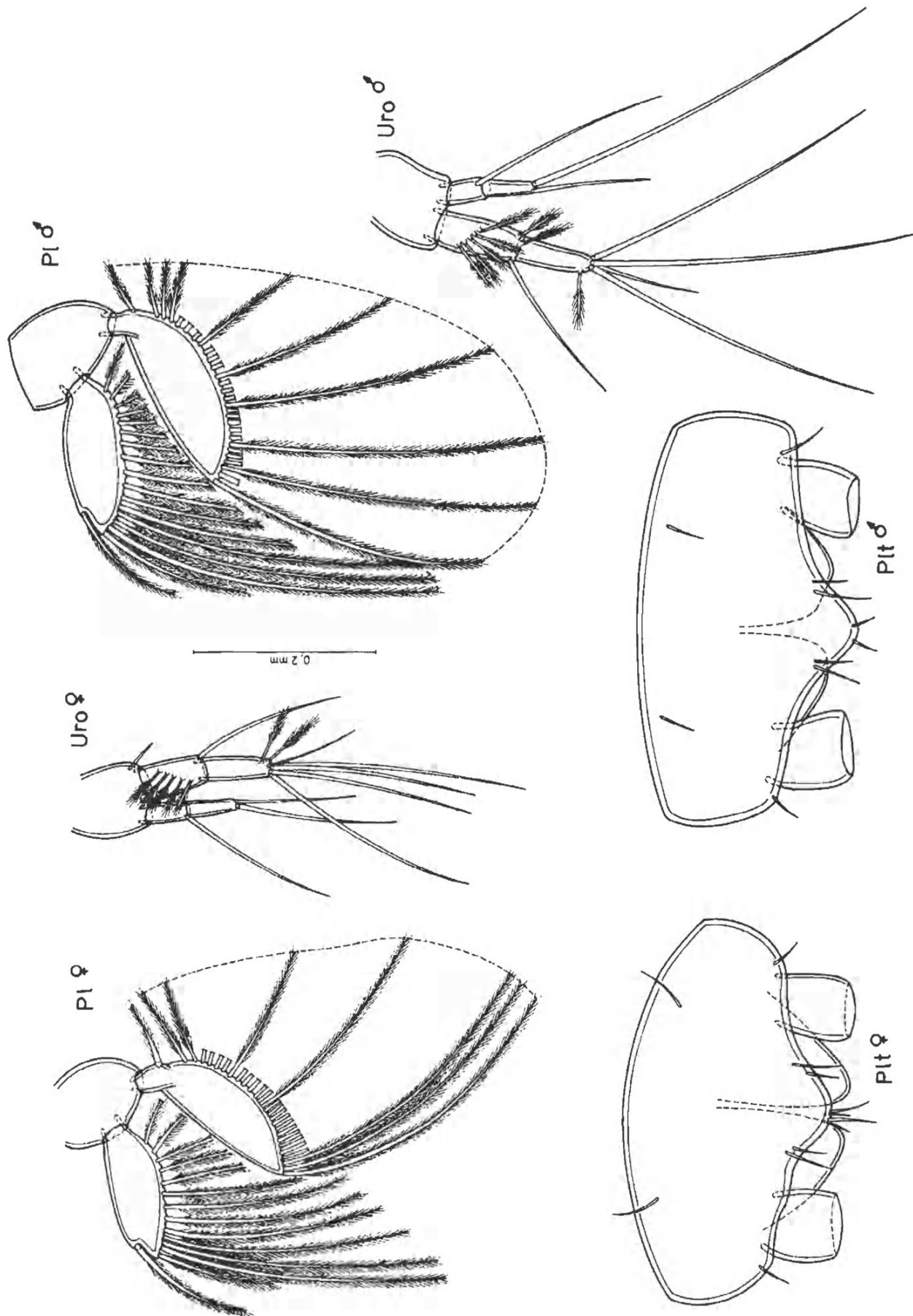
Figure 7. Nototanoides trifurcatus gen. nov., sp. nov. Female and male pleopods (Pl), uropods (Uro), and pleotelson (Plt).
