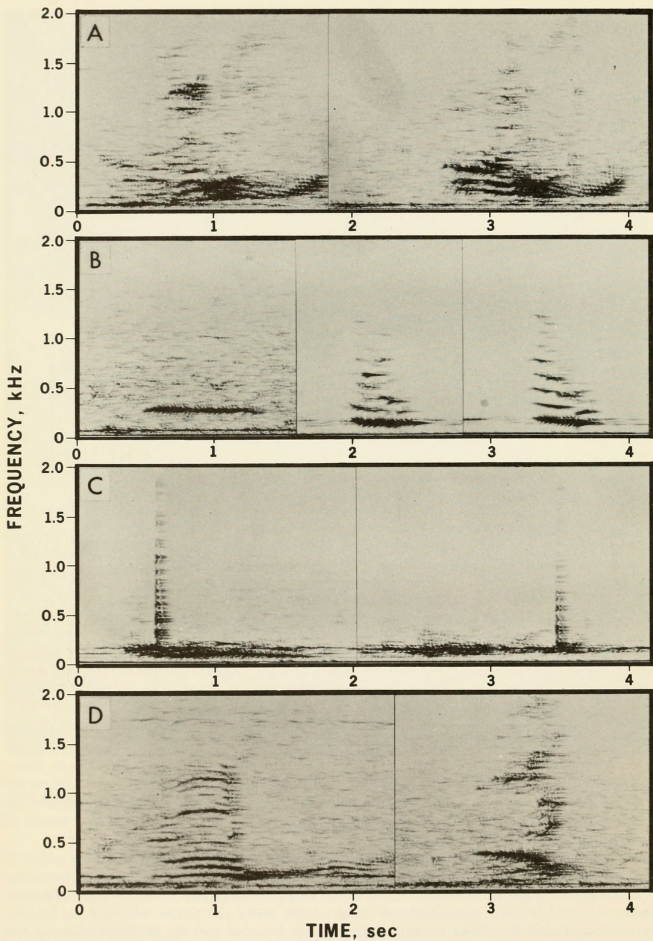
Figure 4. Sonagrams of sounds from southern right whales recorded in Golfo San José, Argentina. Row A, two belch-like sounds; Row B, one simple and two complex moans ; Row C, pulses associated with simple moans ; Row D, two examples of miscellaneous sounds. The effective bandwidth of the analyzing filter for these sonagrams was 10 Hz.
