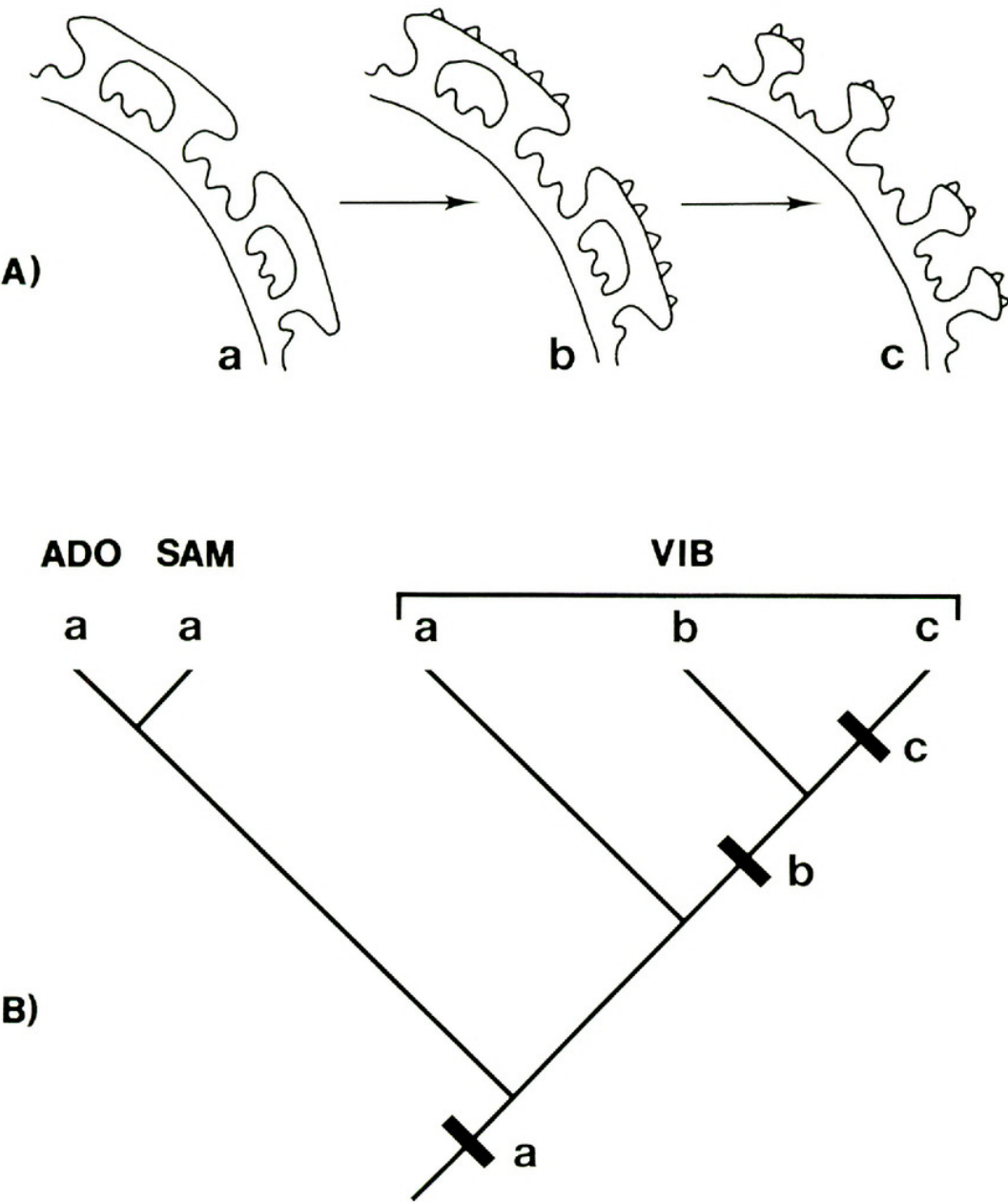
FIGURE 2. A, hypothesized transformation of pollen structure-sculpture classes a, b, and c within Viburnum (all size-shape class I). B, simplest a priori phylogenetic hypothesis for evolution of pollen in Viburnum (VIB), with Sambucus (SAM) and Adoxa (ADO) as first outgroup.
