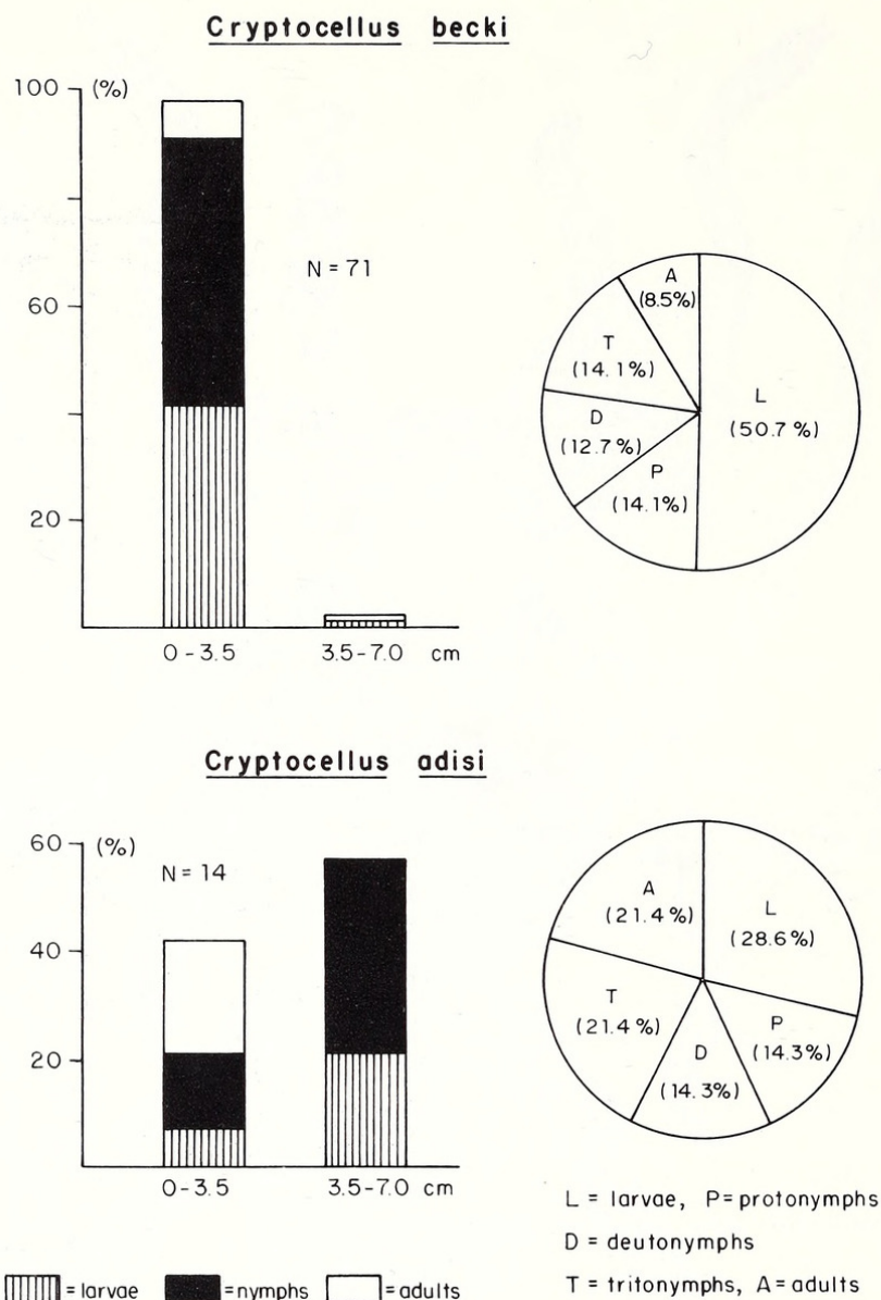
Fig. 3. Distribution of Cryptocellus becki and Cryptocellus adisi in the soil according to soil depth, and percentage of all developmental stages in the secondary dryland forest at Rio Tatumã Mirim near Manaus. (Total catch = 100% for each species.) Samples taken monthly at 0–3.5 and 3.5–7 cm depths between August, 1982 and August, 1983. N = total number of specimens.
