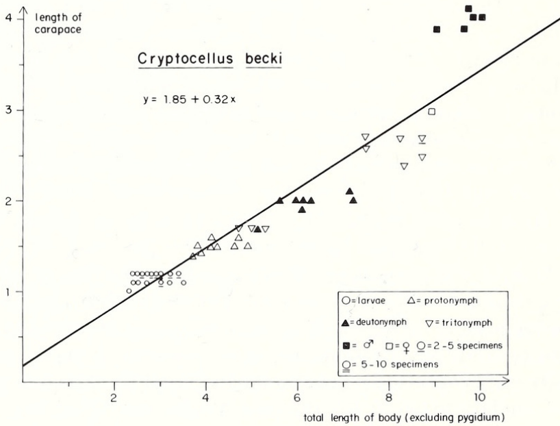
Fig. 5. Relation between length of carapace and total length of body during post-embryonic growth of Cryptocellus becki (1 gradation = 0.6 mm). Seventy-one specimens extracted from soil samples taken monthly at 0–7 cm depth between August, 1982 and August, 1983 in a secondary dryland forest at Rio Taramã Mirim near Manaus (cf. Fig. 4).
