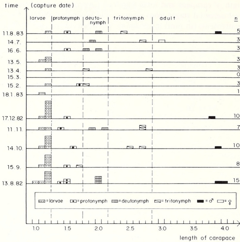
Fig. 4. Developmental stages of Cryptocellus becki extracted from soil samples of a secondary dryland forest at Rio Taramã Mirim near Manaus. Data arranged by length of carapace (1 gradation = 0.6 mm) and capture date. Samples taken monthly at 0–7 cm depth between August, 1982 and August, 1983. N = total number of specimens caught per month.
