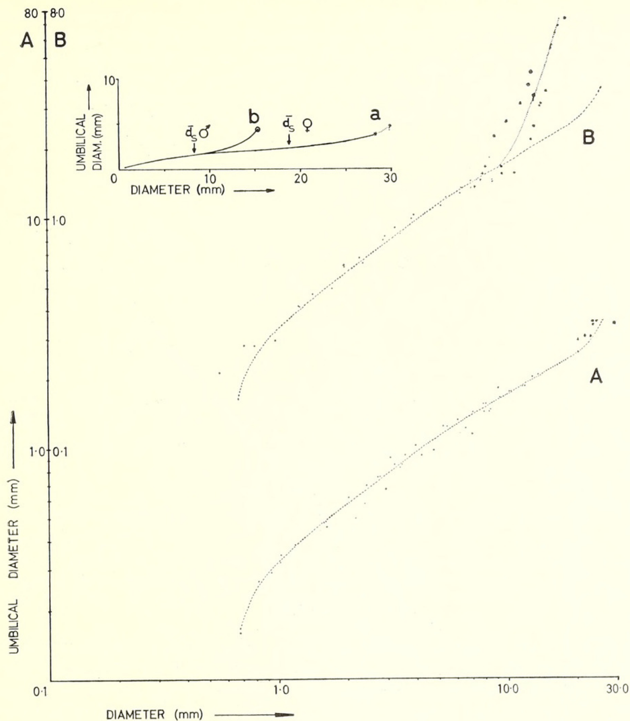
TEXT-FIG. 4. Graphs showing the relationship between diameter and umbilical diameter of Taramelliceras richiei (de Loriol), and of Creniceras renggeri (Oppel). The two graphs are superimposed: the diameter axis is common, the umbilical diameter axis is divided into A and B scales, the B scale being one log cycle behind the A scale. Graph A (U/D for T. richiei ) is controlled by the A scale, graph B (U/D for C. renggeri ) is controlled by the B scale. The fine dashed line on graph B is that superimposed from graph A (approximate best-fit line). Conventions as for text-fig. 3.
