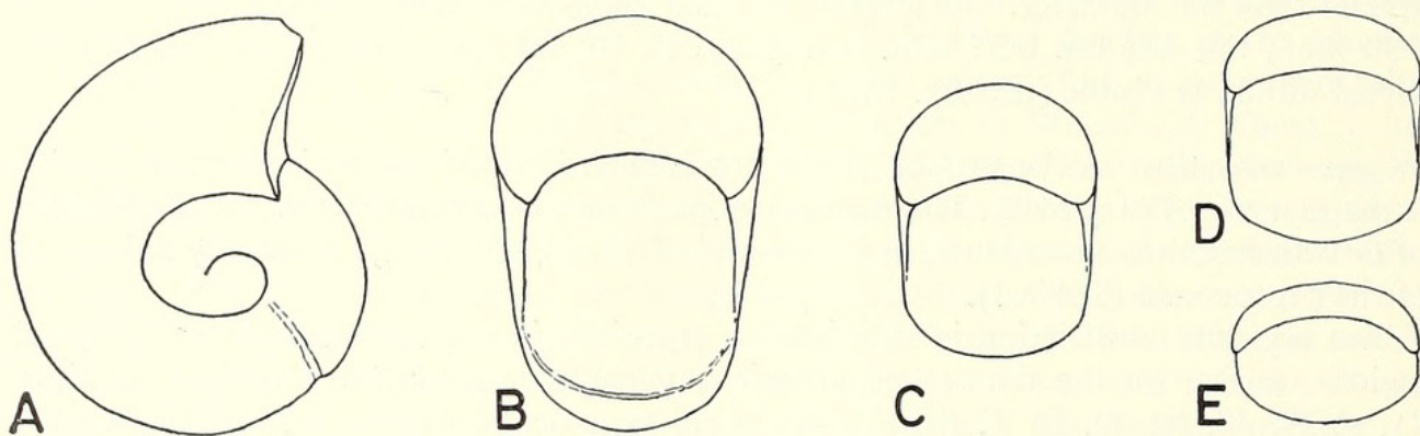
TEXT-FIG. 2. Diagram of the innermost whorls of Taramelliceras richei (de Loriol); Mariae Zone, Woodham, Bucks., England. A and B, showing the position of the nepionic constriction; C, protoconch. A, B, C, and D, drawn from OUM J25038; E, drawn from OUM J25234. All \times 50 .
