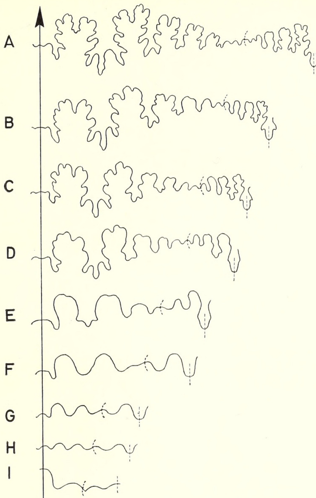
TEXT-FIG. 12. Sutural ontogeny of Creniceras renggeri (Oppel). A, OUM J25244, \times 12 ( D_1' = 10.61 mm.); B, OUM J25364, \times 15 ( D = 8.03 mm.); C, OUM J25364, \times 16 ( D = 6.08 mm.); D, OUM J25364, \times 25 ( D = 3.18 mm.); E, OUM J25364 \times 50 ( D = 1.43 mm.); F, OUM J25364, \times 50 ( D = 0.99 mm.); G, OUM J25364, \times 50 ( D = 0.38 mm.); H, OUM J25364, \times 50 ( D = 0.33 mm.); I, OUM J25364, \times 50 ( D = 0.28 mm.). H, primary suture. I, prosuture. All specimens from the Mariae Zone, Woodham.
