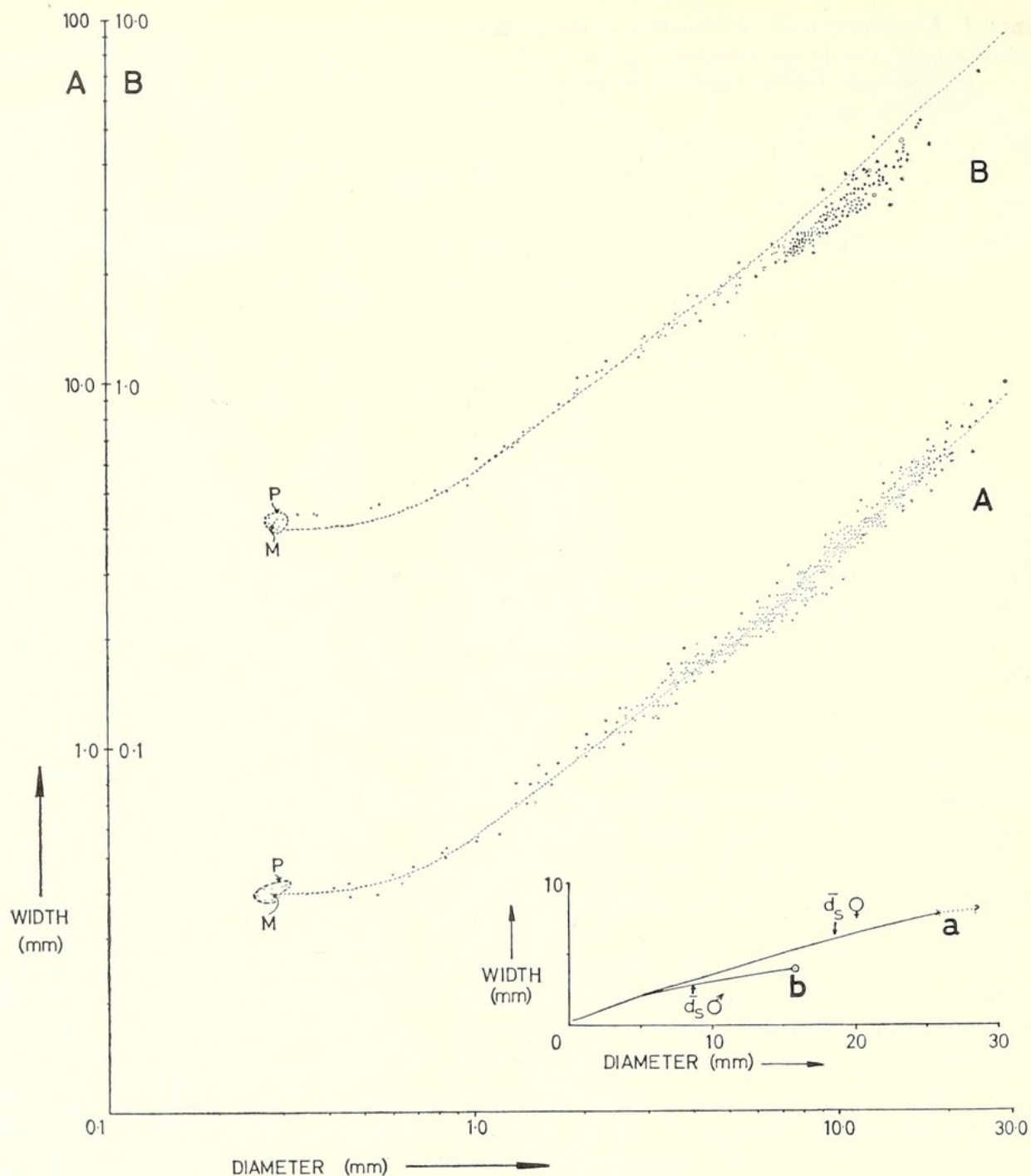
TEXT-FIG. 3. Graphs showing the relationship between diameter and whorl width of Taramelliceras richei (de Loriol), and of Creniceras renggeri (Oppel). The two graphs are superimposed: the diameter axis is common, the width axis is divided into A and B scales, the B scale being one log cycle behind the A scale. Graph A (W/D for T. richei ) is controlled by the A scale, graph B (W/D for C. renggeri ) is controlled by the B scale. The fine dashed line on graph B is that superimposed from graph A (approximate best-fit line). The areas denoted by P (coarse dashed line) enclose measurements made on the protoconchs: M is the mean of these measurements. Encircled dots represent measurements made at the maximum diameter of complete adults: asterisks—measurements made on adult body-chambers: crosses—measurements made at the adoral end of adult phragmocones: dots—measurements made on immature phragmocones.
