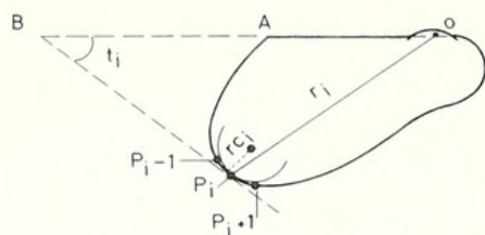
TEXT-FIG. 2. Measurements on a shell outline. The hinge OA is produced to B . P_{i-1} , P_i , P_{i+1} are three consecutive points on the outline. rc_i is the radius of curvature, t_i the tangent angle, and r_i the distance from O of point P_i .
