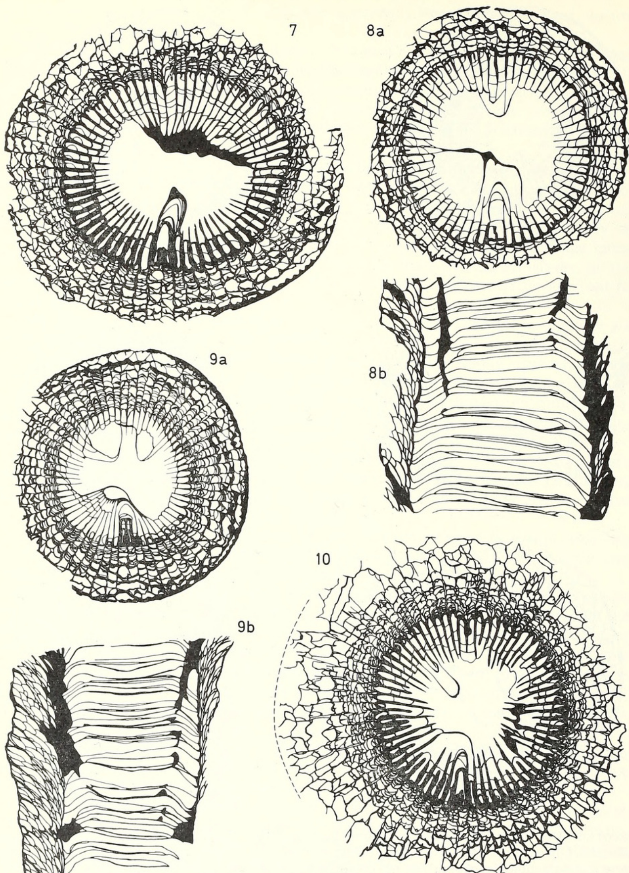
TEXT-FIGS. 7-10. Caninia benburbensis . 7. Form B. C. 7475b. Transverse section. Epithea mostly obscured by silicification. 8a, b. Intermediate form B-C. C. 7476b, C. 7476d. Transverse and longitudinal sections. 9a, b. Form C. C. 7477d, C. 7477b. Transverse and longitudinal sections. Specimens represented by text-figs. 8 and 9 both show the effects of penecontemporaneous abrasion. 10. Form D. C. 7478i. Transverse section. Dissepimentarium partly abraded. Silicified epithea approximately at dashed line.
