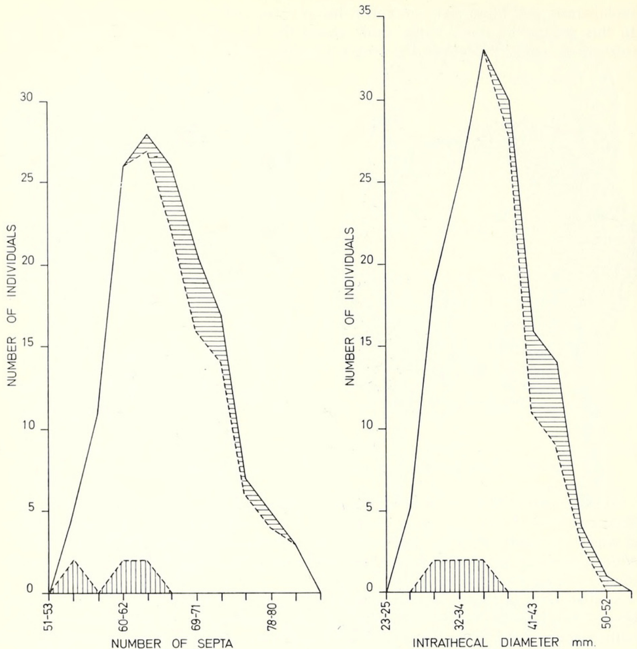
TEXT-FIGS. 12-13. Frequency curves of Caninia benburbensis . Vertical and horizontal ruling represents the frequency of Form A and Form D, respectively.
