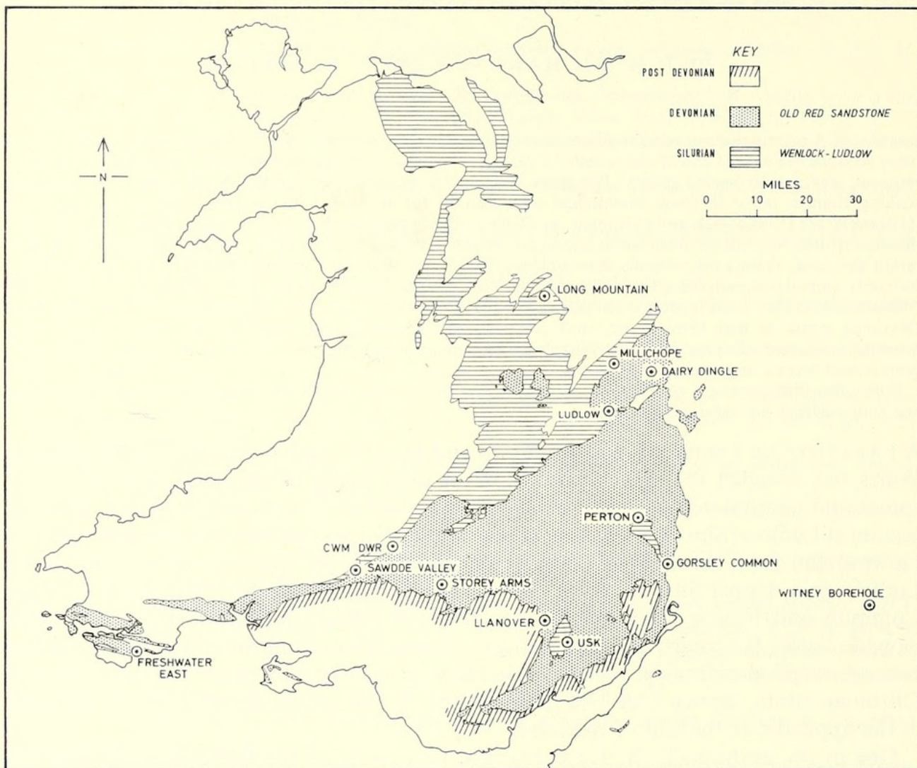
TEXT-FIG. 1. Location of the main sampling areas.
