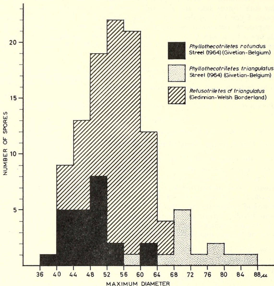
TEXT-FIG. 3. Size distribution of Retusotriletes cf. triangulatus (Streel) from the Dittonian of the Welsh Borderland compared with Streel's data from the Lower Givetian of Goé, Belgium (Streel 1964).
