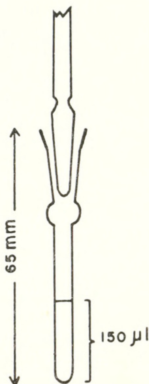
FIGURE 3. Micro-homogenizer constructed from a 5/20 Pyrex interconnecting joint.
