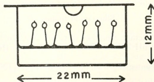
FIGURE 2. Diffusion cell with hanging drop of 0.01 N \text{H}_2\text{SO}_4 to absorb \text{NH}_3 liberated by the slime molds.
