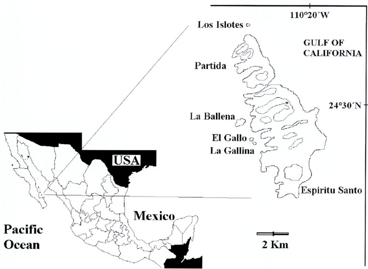
FIG. 1. Geographical location of the study area in northwestern Mexico, at the Gulf of California insular system. Isolines indicate areas over 200 m. Cross (+) indicates the highest point in the island (540 m).
