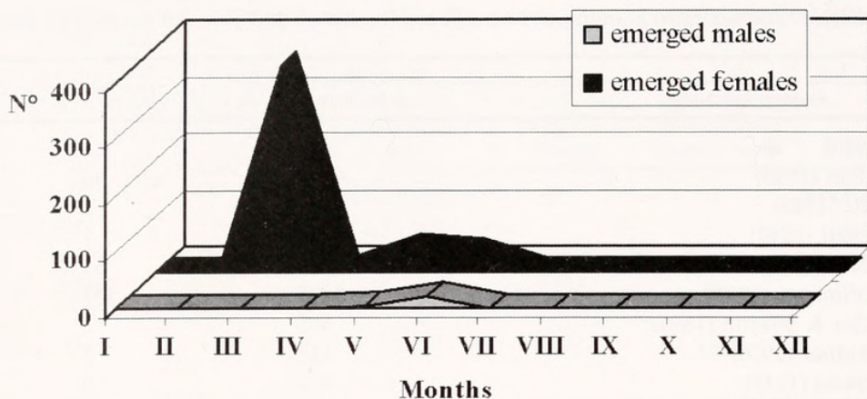
Fig. 1. Seasonal appearance of adults of D. rosae in Sicily.
