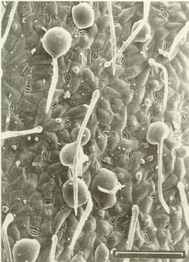
Fig 2. Scanning electron micrograph of the lower surface of leaflets in Ac. marashica (isotype: MSB). Scale bar: 200 \mu m.
