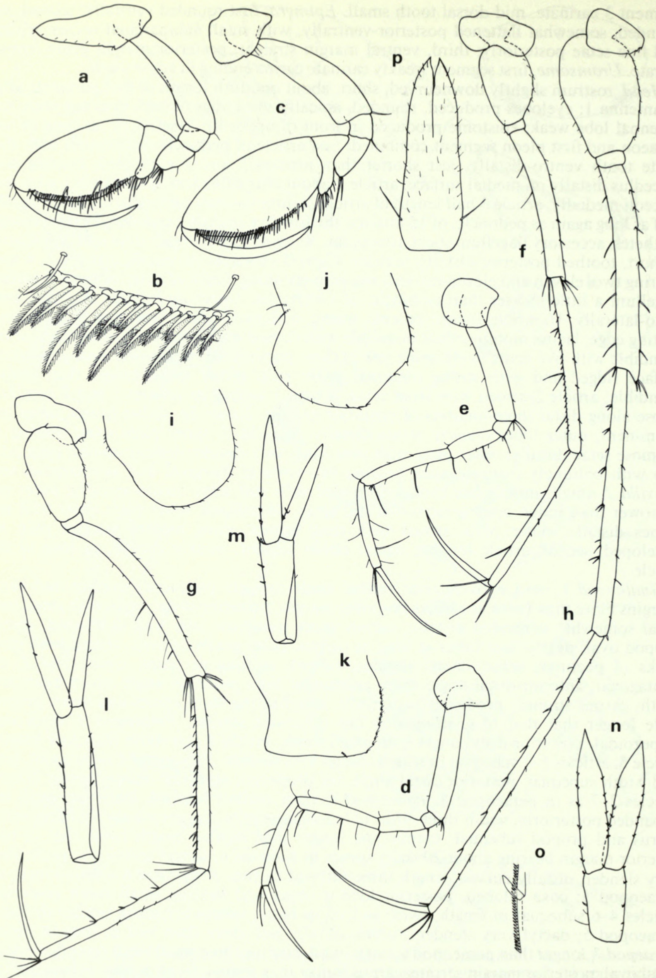
Fig. 4 Rhachotropis thordisae sp. nov. Holotype, male, 9mm. (a) gnathopod 1; (b) gnathopod 1, detail of palm; (c) gnathopod 2; (d-h) pereopods 3-7; (i-k) epimera 1-3; (l-n) uropods 1-3; (o) uropod 3, margin of outer ramus; (p) telson.
