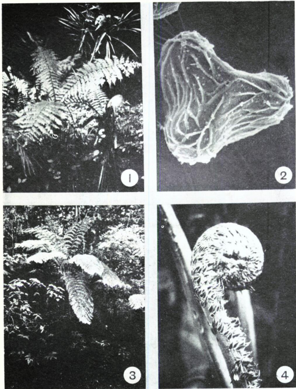
Figs. 1-2. Alsophila dryopteroides \times Nephelea portoricensis : 1, plant, stem ca. 75 cm. tall, leaves ca. 1.0 m. long, Conant 679; 2, spore, \times 1500, Conant 687. Figs. 3-4. Cnemidaria horrida \times Cyathea arborea : 3, plant, stem ca. 2.0 m. tall, leaves ca. 2.5 m. long, Conant 626; 4, bicolorous scales on crozier, \times 1/3, Conant 546. (all specimens GH).
